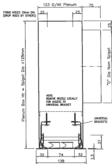
Universal Bracket Arrangement
